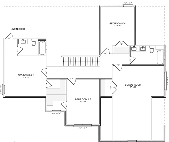
2ND FLOOR
