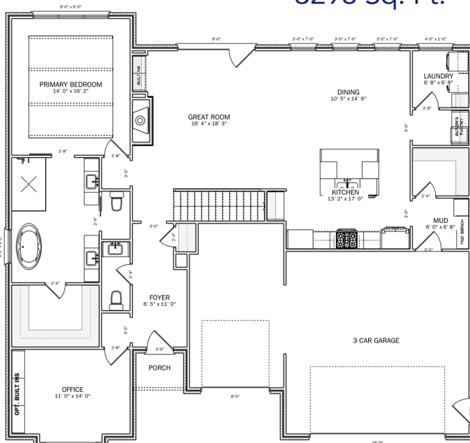
MAIN FLOOR
